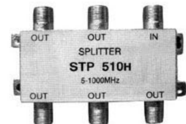
5-Way Splitter Model:STP510
